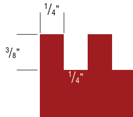
620312 1/4'' \times 1/4'' \times 3/8''
