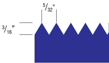
620306 3/16'' \times 5/32''
