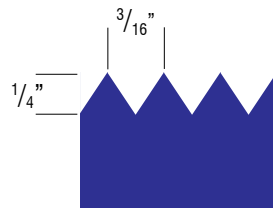
620308 1/4'' \times 3/16''
